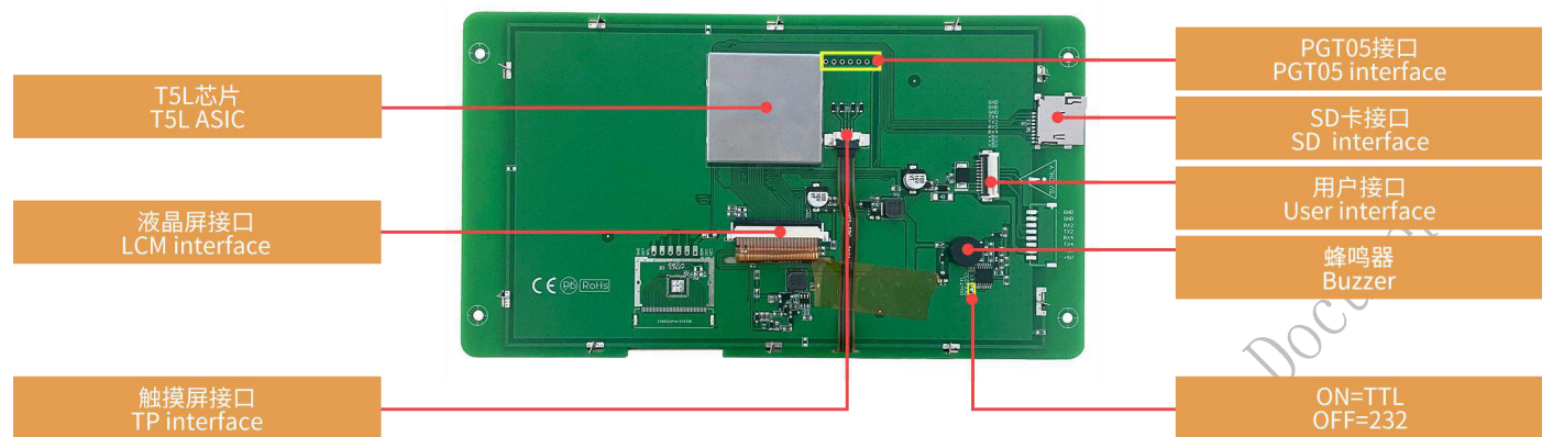
硬件接口图 Hardware interface
