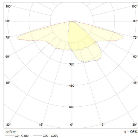
CREE XPG3
