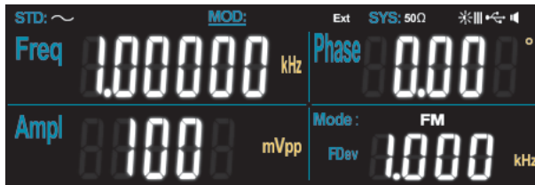
Picture 4-11 Select FM modulation source
