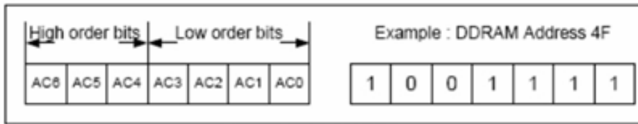
Figure 7. DDRAM Address
