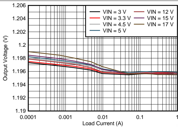
Figure 30. Line and Load Regulation V_{OUT} = 1.2\text{ V}
