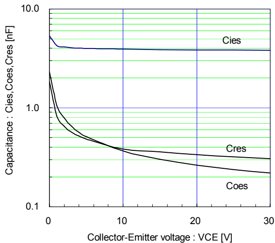
[ Brake ] Capacitance vs. Collector-Emmitter voltage (typ.) VGE=0V, f= 1MHz, Tj= 25°C
