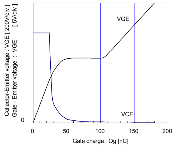
[ Brake ] Dynamic Gate charge (typ.) Vcc=600V, Ic=50A, Tj= 25°C
