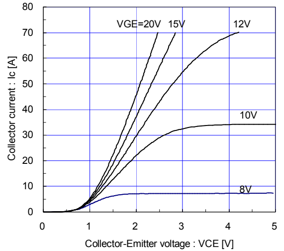
[ Brake ] Collector current vs. Collector-Emmitter voltage (typ.) Tj= 125°C / chip
