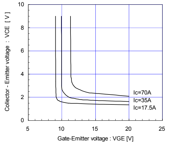
[ Brake ] Collector-Emmitter voltage vs. Gate-Emmitter voltage (typ.) Tj=25°C / chip
