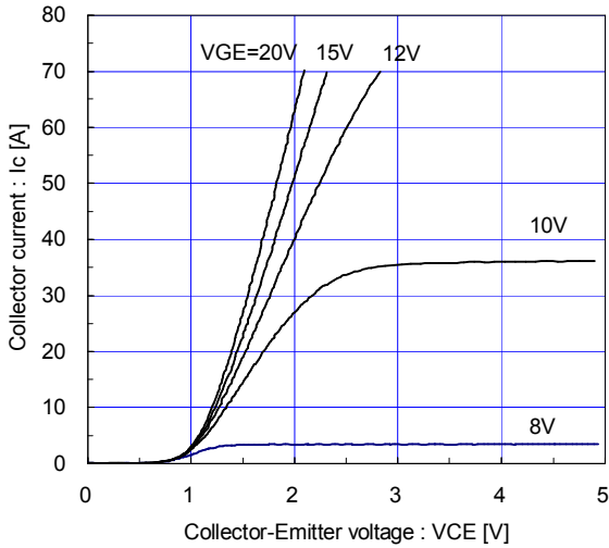
[ Brake ] Collector current vs. Collector-Emmitter voltage (typ.) Tj= 25°C / chip
