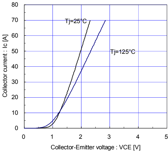
[ Brake ] Collector current vs. Collector-Emmitter voltage (typ.) VGE=15V / chip
