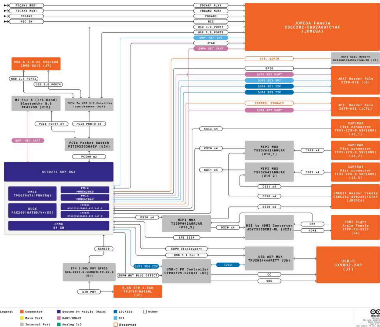
Block Diagram (Page 2/2)
