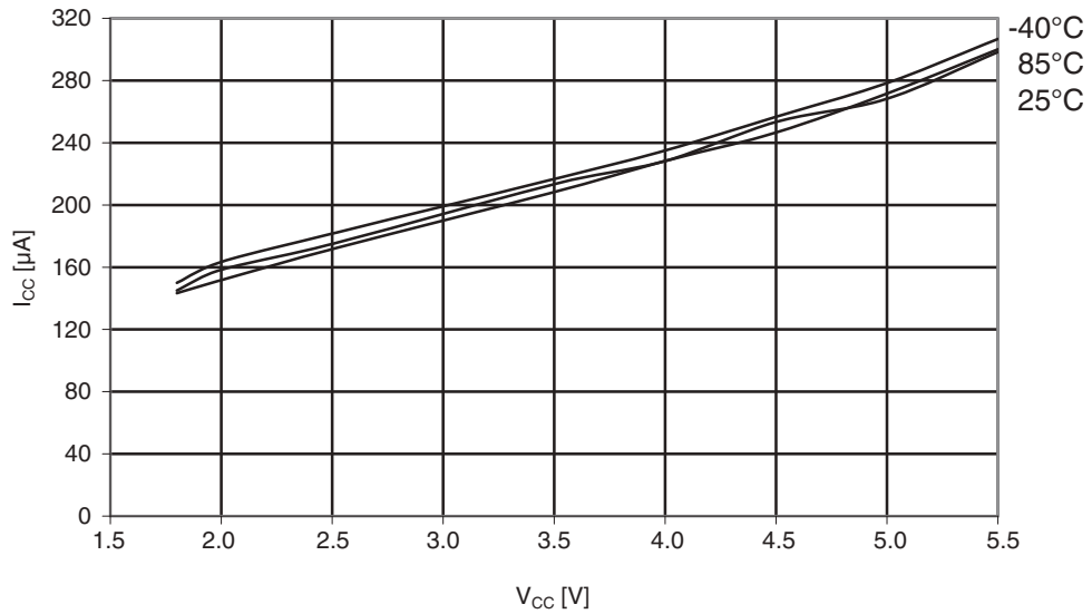
Figure 30-90. Atmel ATmega164PA: ADC current vs. V_{CC} (AREF = AV_{CC} ).
