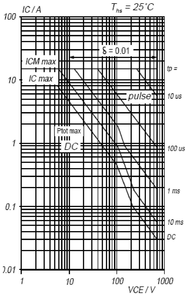
Safe Operating Area
