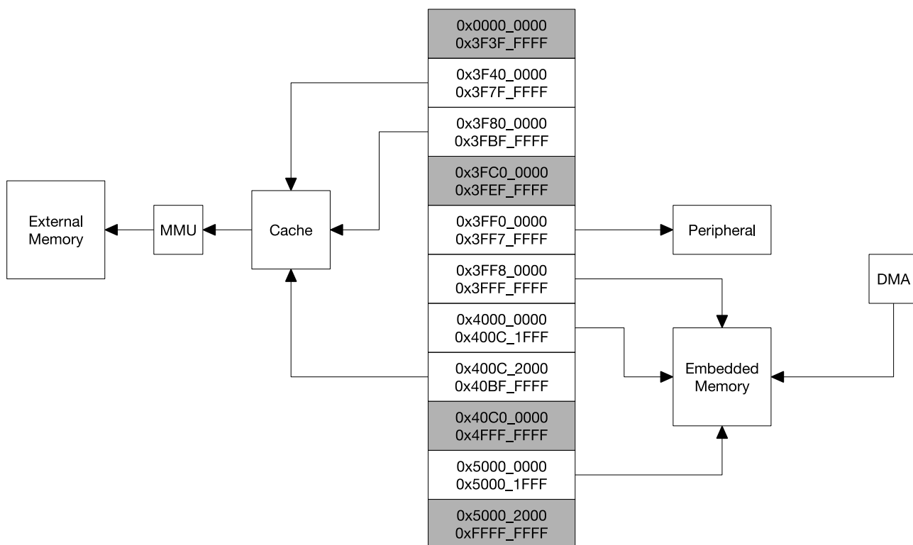
Figure 5: Address Mapping Structure
