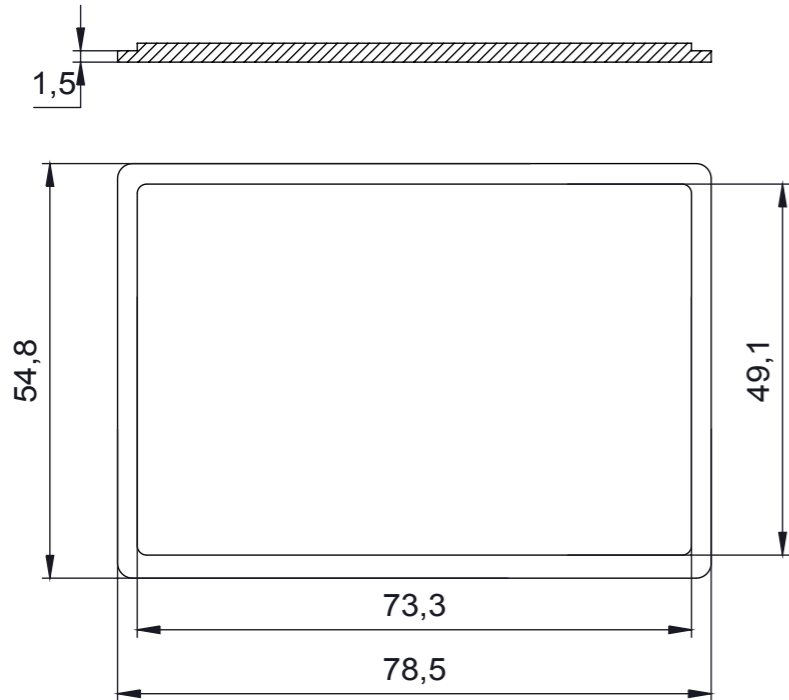
HH-8282 Panel
