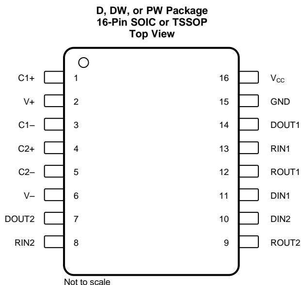
Pin Functions
