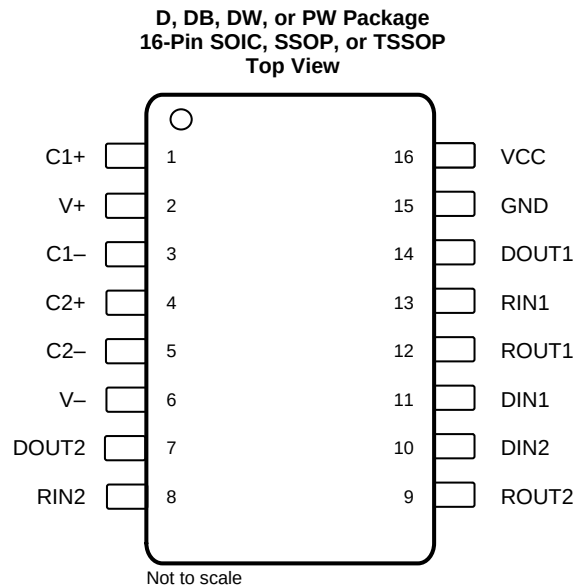
Pin Functions
