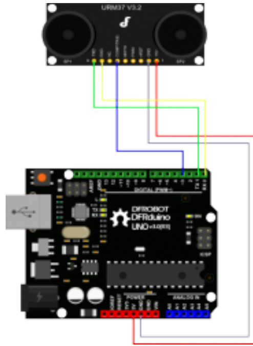
• TTL Mode Connection Diagram
