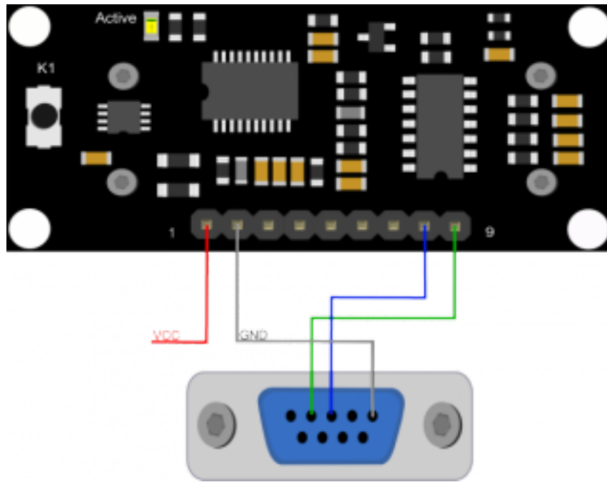
• RS232 Mode Connection Diagram
